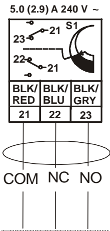
Figure 5: Optional Auxiliary Switch Wiring
