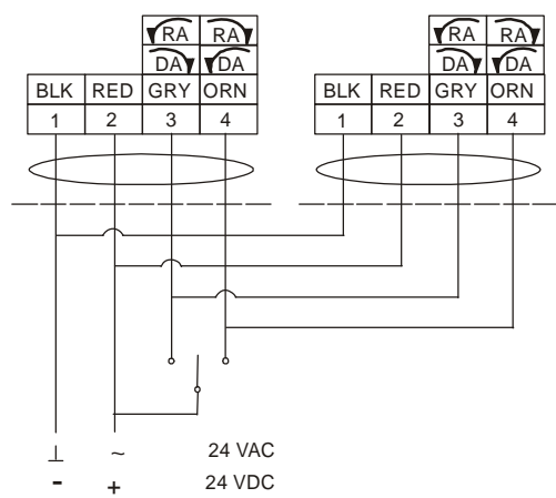
Figure 6: VA9203-AGx-2Z Control Wiring Diagrams
