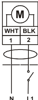
Figure 4: VA9203-Bxx-2 Control Wiring Diagrams
